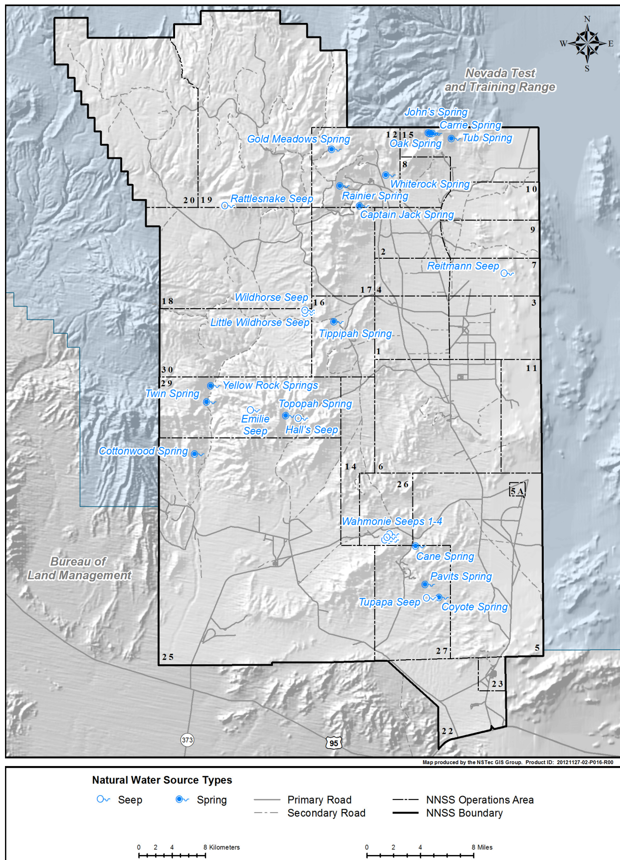
Figure A-4. Natural springs and seeps on the NNSS (adapted from Hall et al. 2013)
