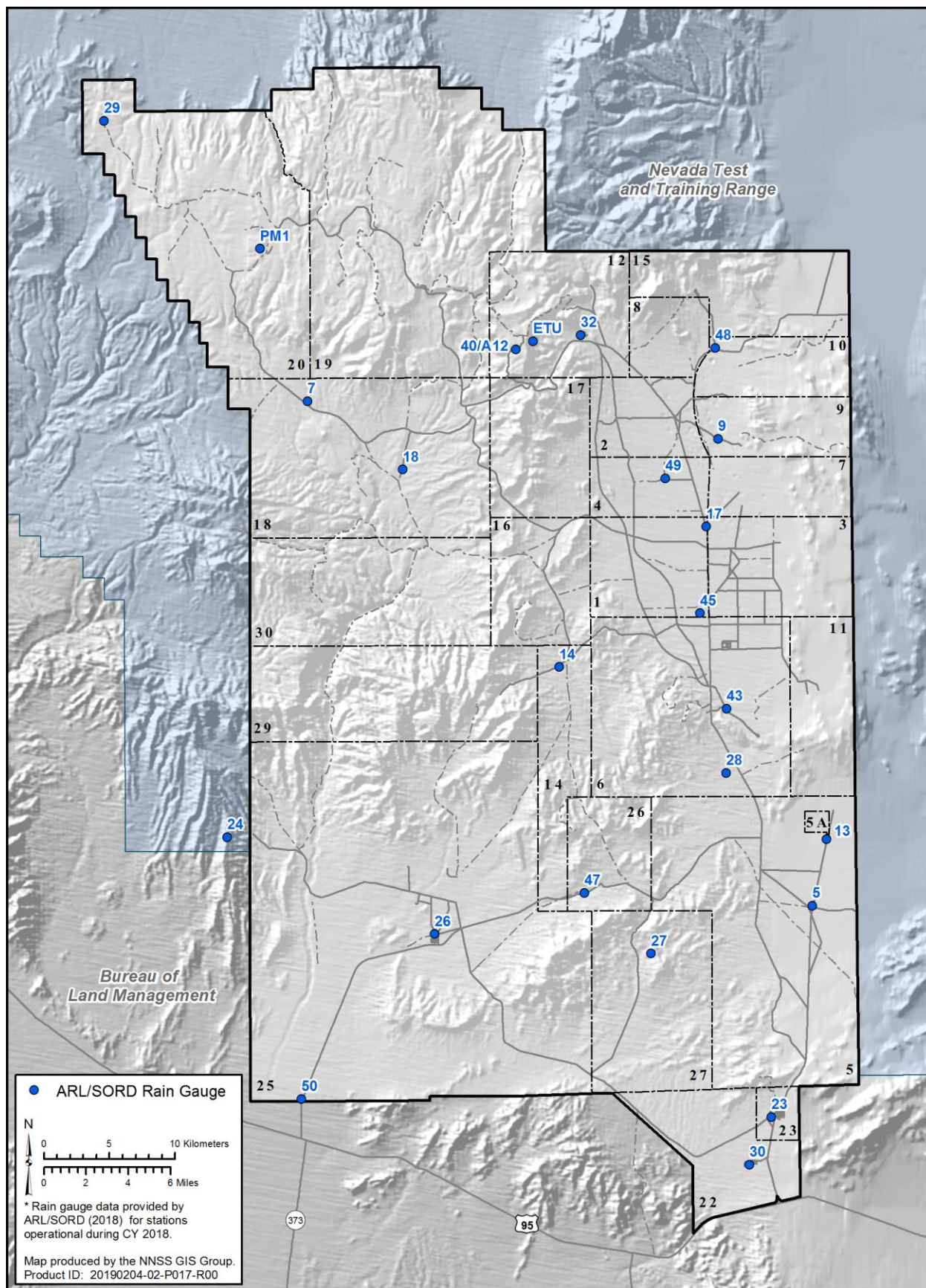
Figure A-15. 2018 climatological rain gauge network on the NNSS
