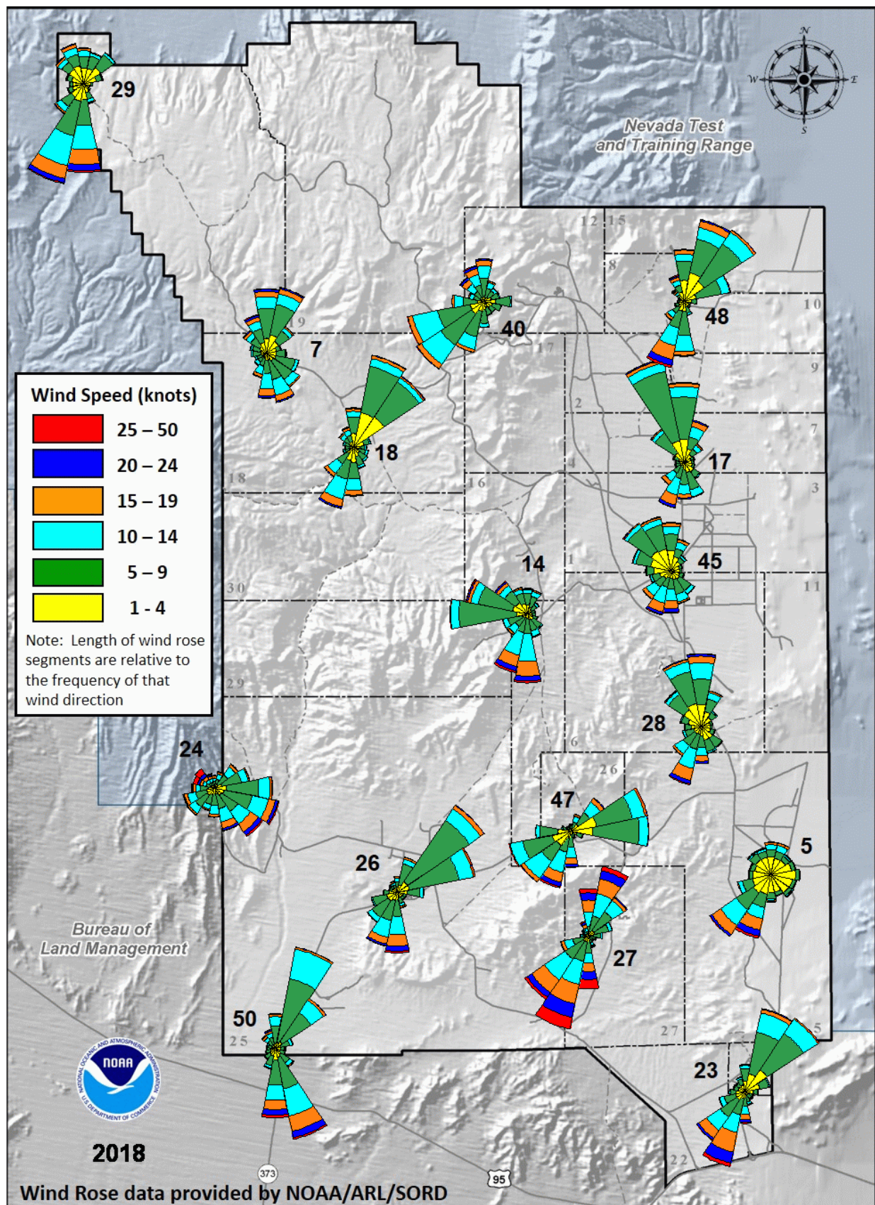
Figure A-18. Annual wind rose climatology for the NNSS (2005–2018)
