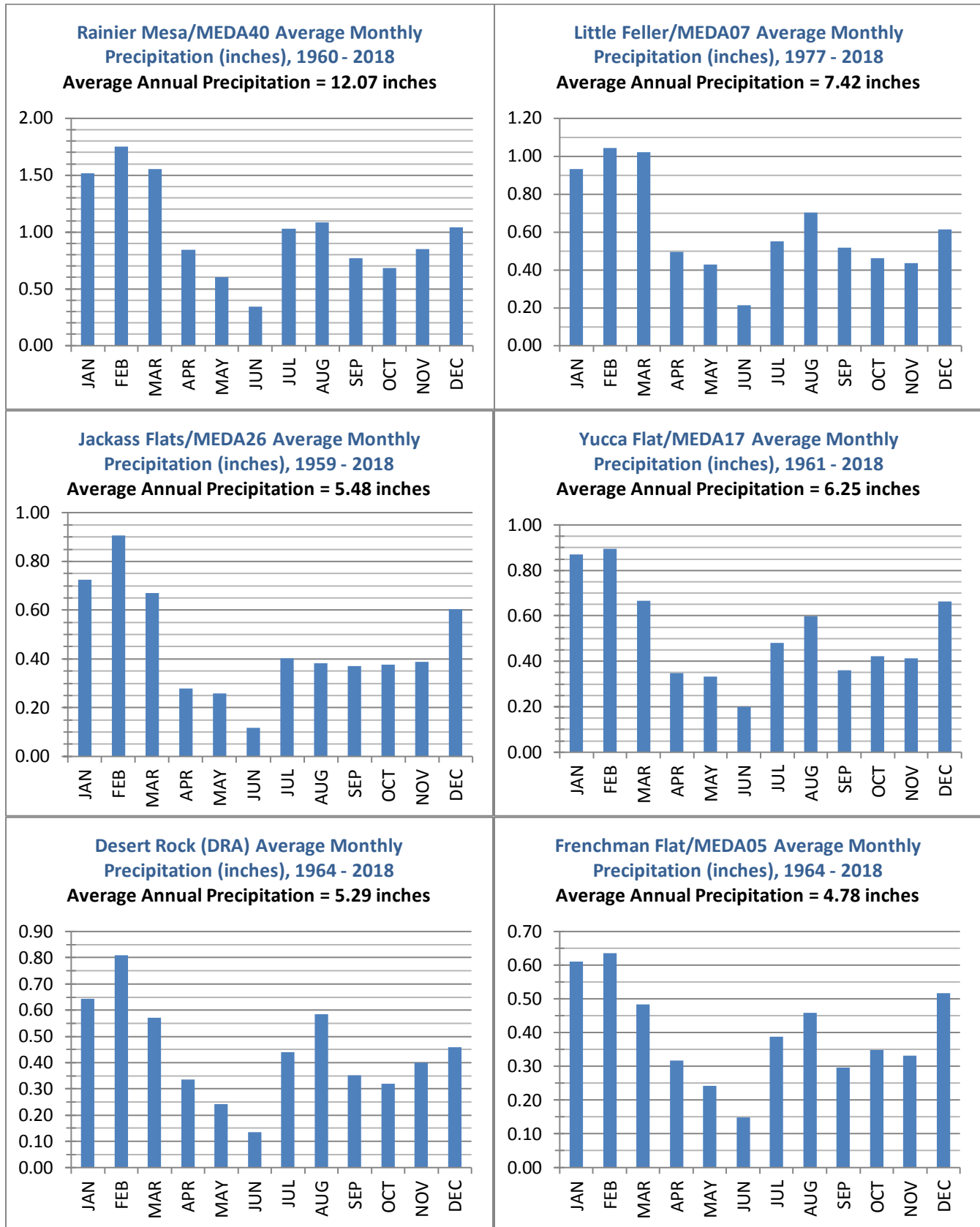
Figure A-16. Mean monthly precipitation at six NNSS rain gauge stations (locations of numbered stations are shown in Figure A-14)
