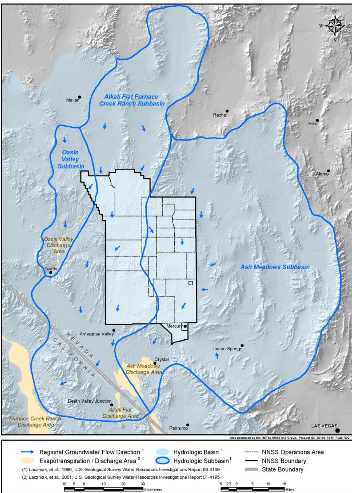
Figure A-5. Groundwater subbasins of the NNSS and vicinity (modified from Waddell et al. 1984; Lacznai et al. 1996, 2001)
