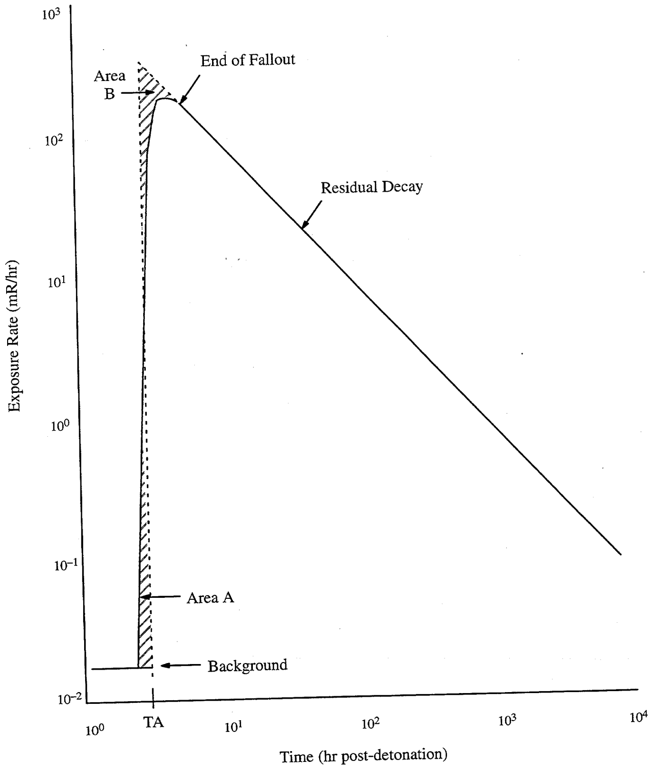
Figure 2. Typical form of an exposure rate profile.
