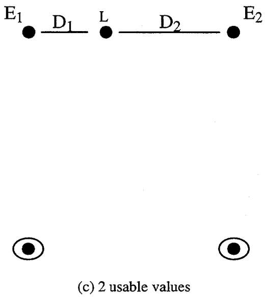
Figure 7. Situations where estimates can be calculated from the 10-km grid. L is the location for which estimates are to be made; the E_i are values interpolated from a fallout pattern at the grid nodes; and D_i is the distance from node i to L . Values at circled grid nodes are not used in the calculation.
