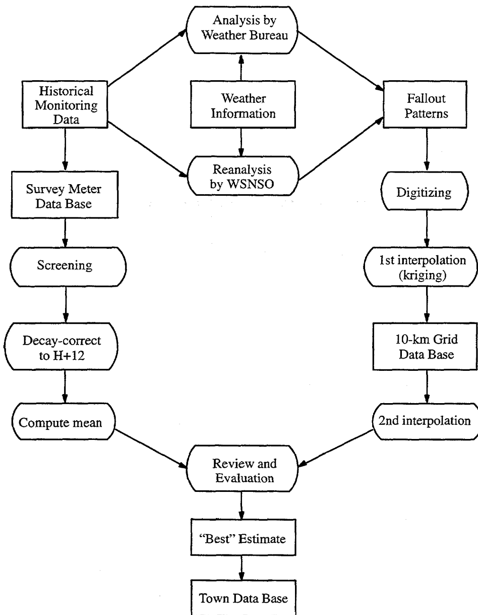
Figure 4. Generalized flow diagram of the estimation process.
