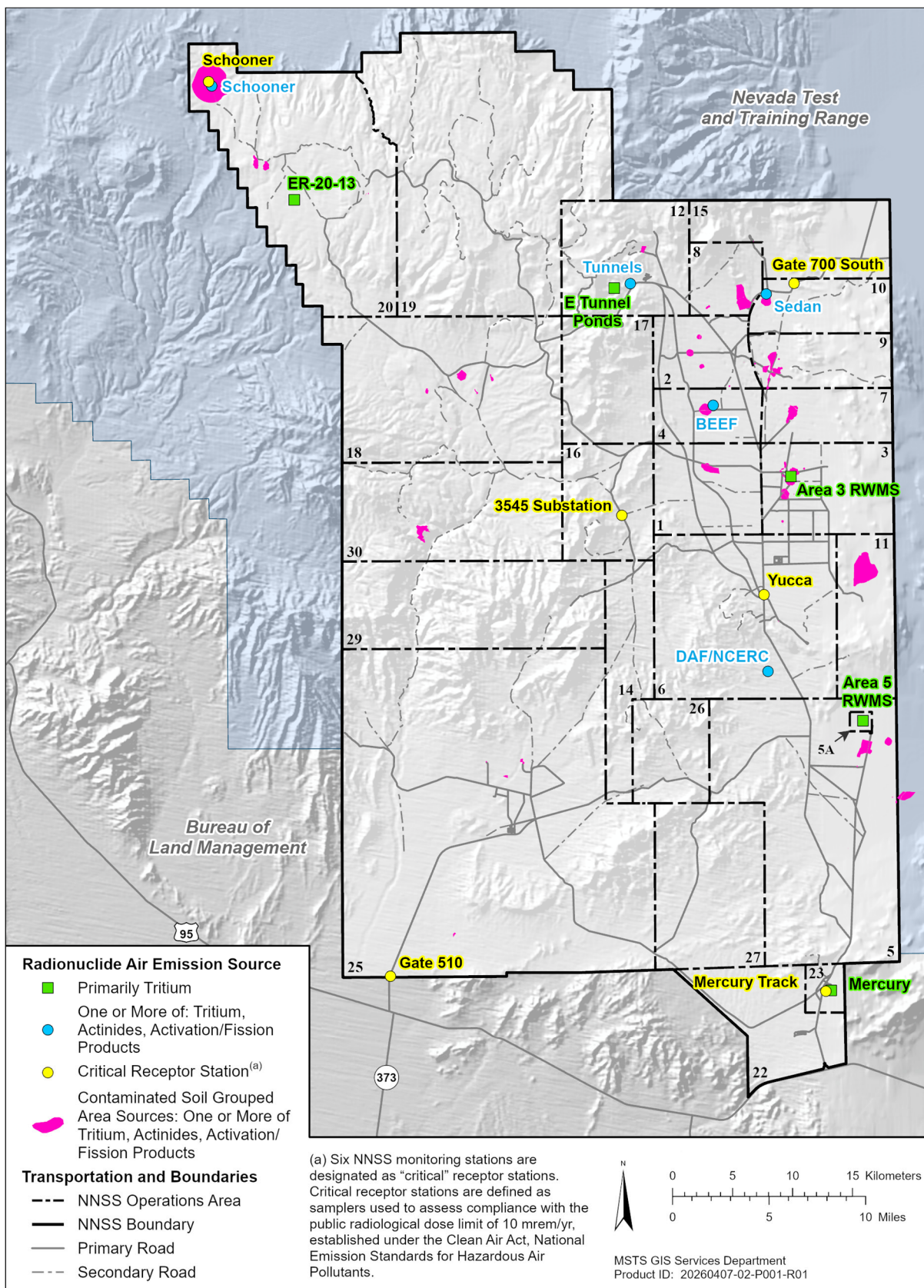
Figure 4. Sources of Radiological Air Emissions and Critical Receptor Air Monitoring Stations on the NNSS in CY 2025
