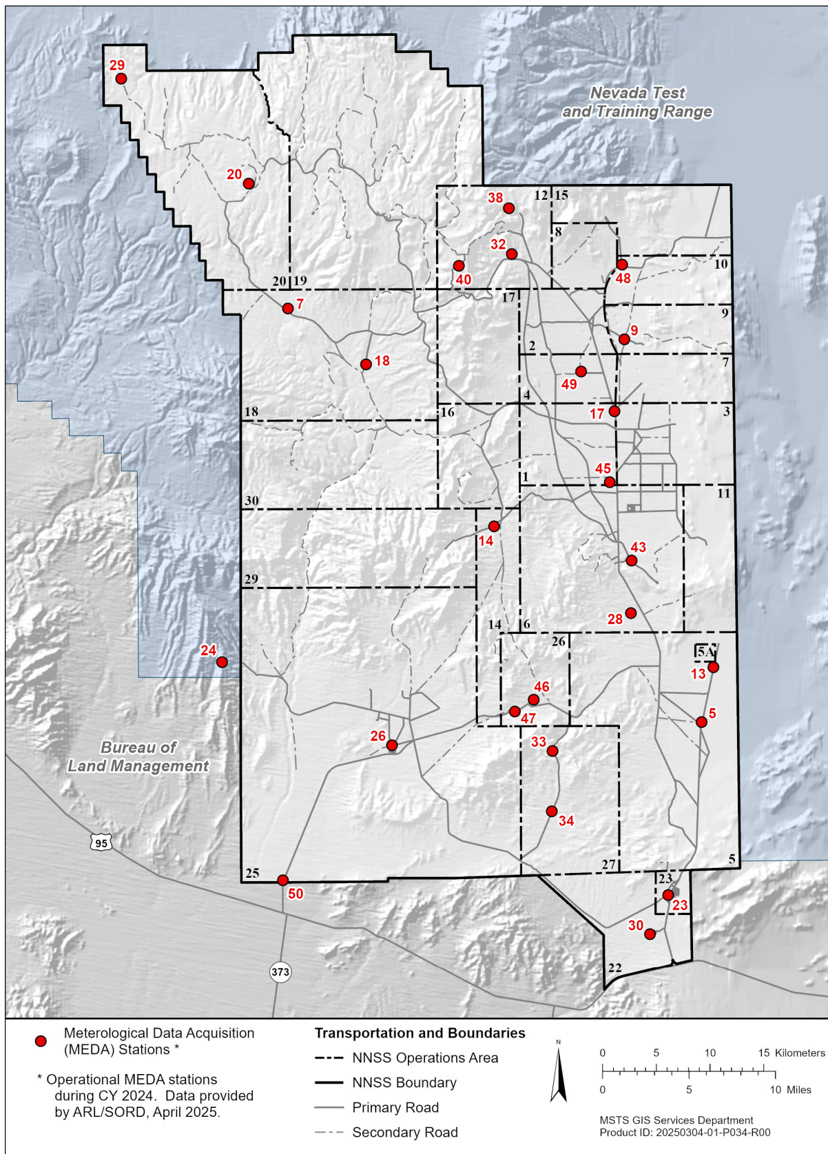
Figure F.1. Locations of MEDA Stations on the NNSS at End of CY 2025
